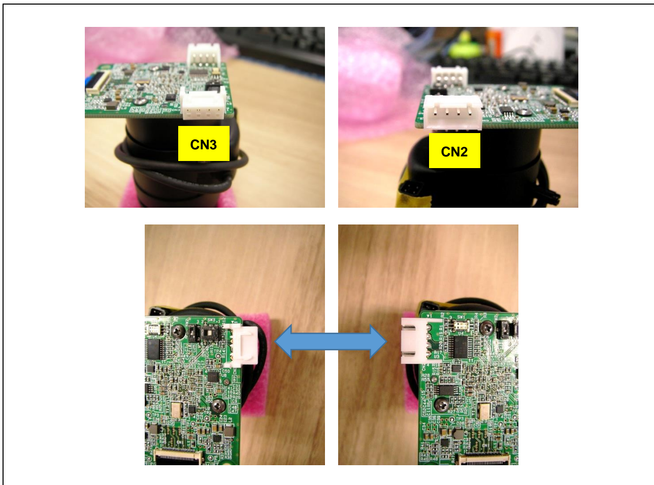
Figure 3.2-1 Connect the on-board connectors of the IMX415 boards.
