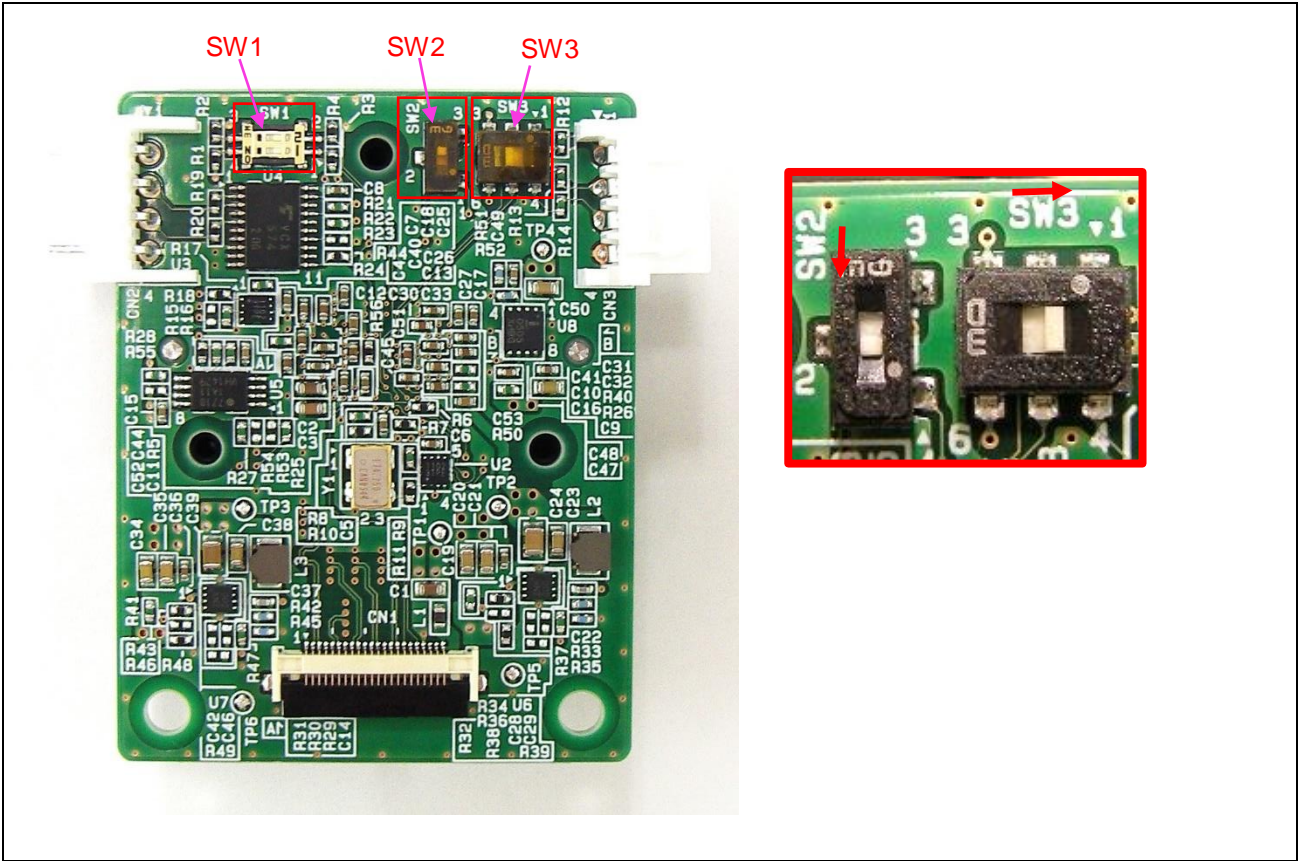
Figure 3.3-1 Switch Setting in Single Sensor Mode
