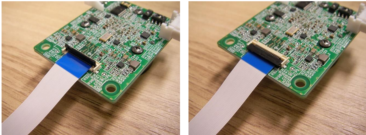
Figure 3.1-1 Connect FFC to IMX415 Board.
