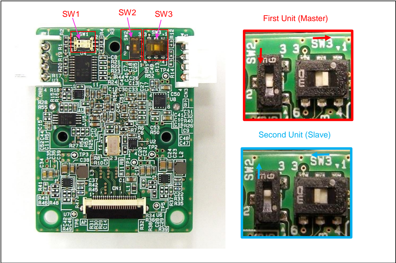
Figure 3.3-2 Switch Setting in Dual Sensor Mode
