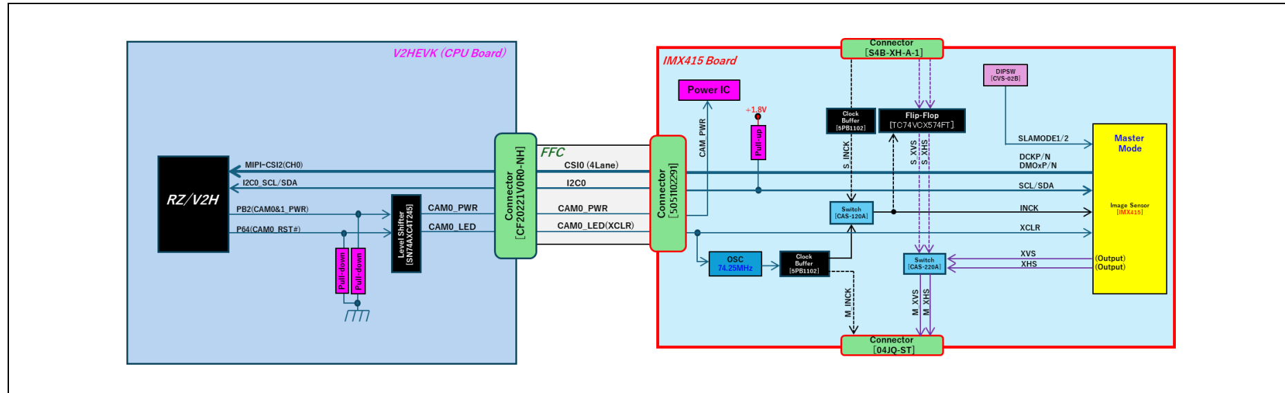
Figure 1.2-1 IMX415 Board Block Diagram (Single Sensor Mode)
