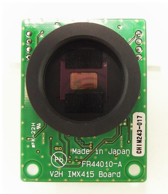
Figure 2.2-3 IMX415 Board (IMX415 sensor side)
