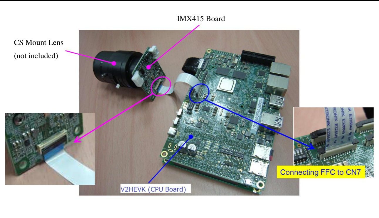
Figure 2.2-1 Outer Appearance of V2HEVK (with IMX415 Board : Single Sensor Mode)
