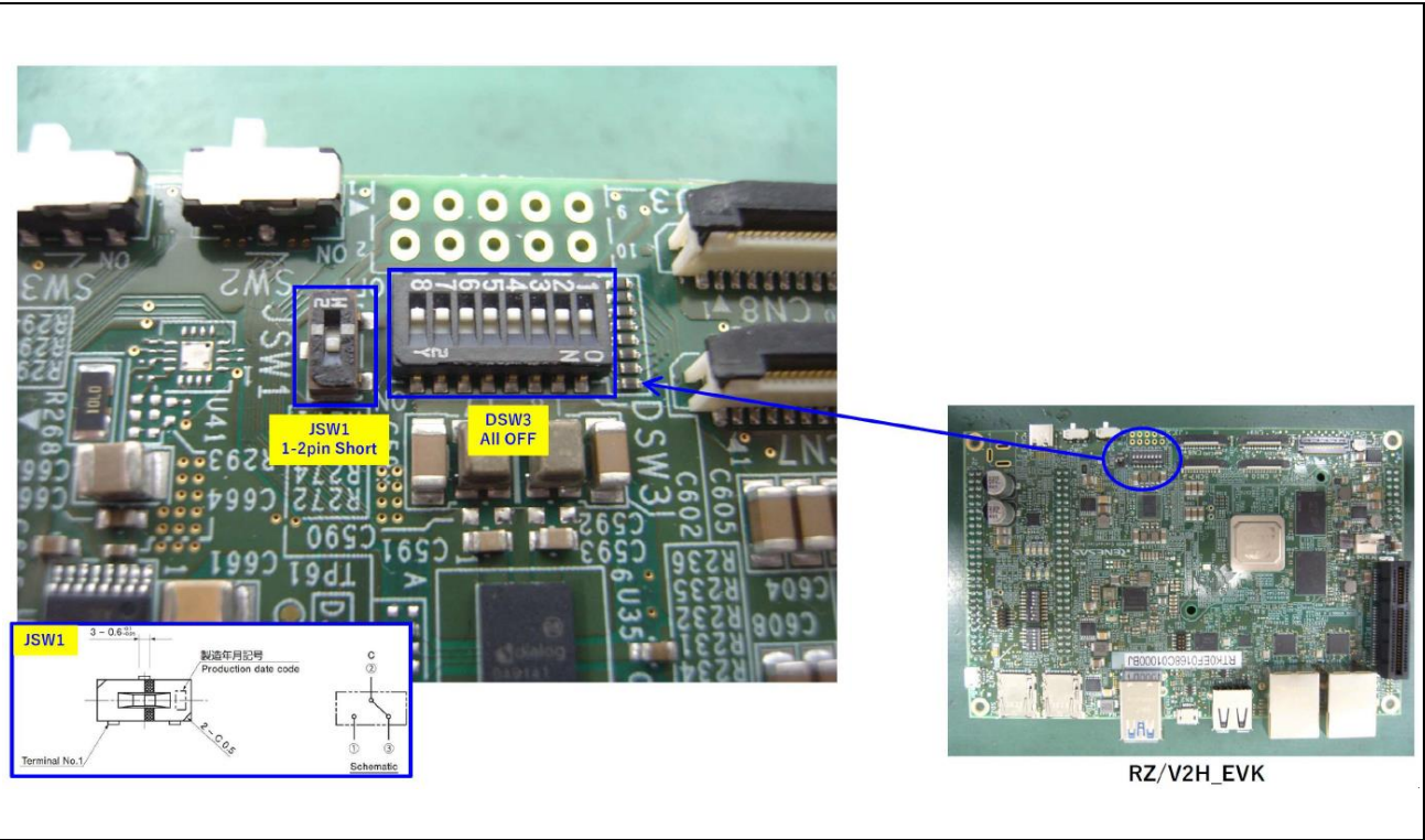
Figure 3.3-3 Switch Setting in RZ/V2H Evaluation Board Kit
