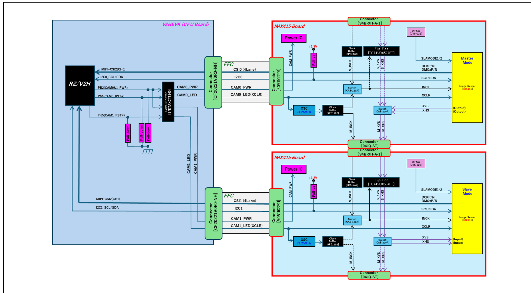
Figure 1.2-2 IMX415 Board Block Diagram (Dual Sensor Mode)
