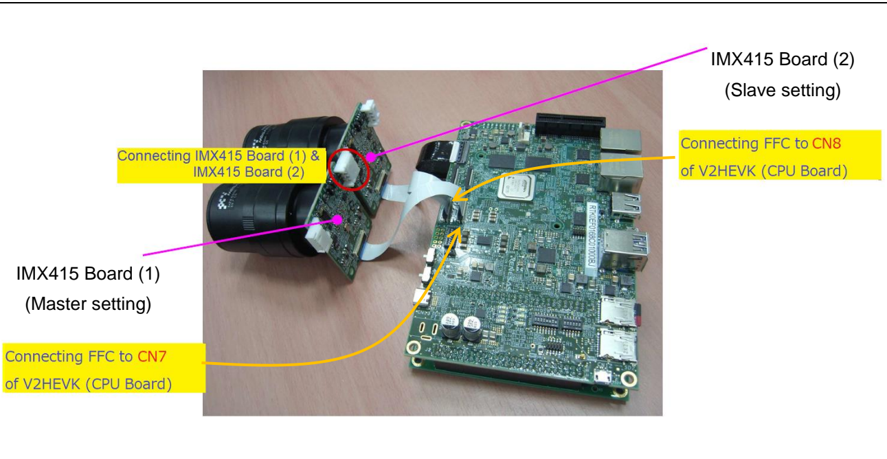
Figure 2.2-2 Outer Appearance of V2HEVK (with IMX415 Board : Dual Sensor Mode)
