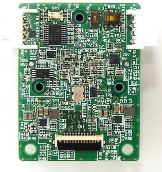
Figure 2.2-4 IMX415 Board (V2HEVK connector side)
